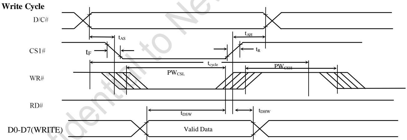
Figure 12-3 : Parallel 8080-series Interface Timing Characteristics
