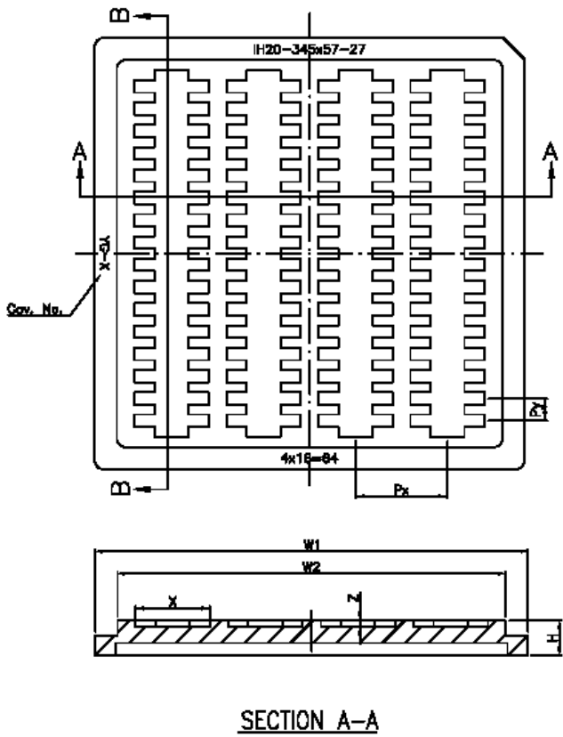
Figure 14-1 : SSD1603Z die tray information
