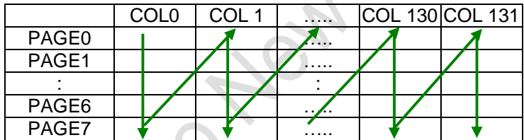
Figure 9-3 : Address Pointer Movement of Vertical addressing mode
