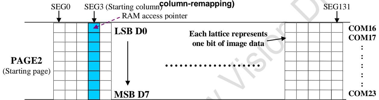
Figure 9-1 : Example of GDDRAM access pointer setting in Page Addressing Mode (No COM and column-remapping)
