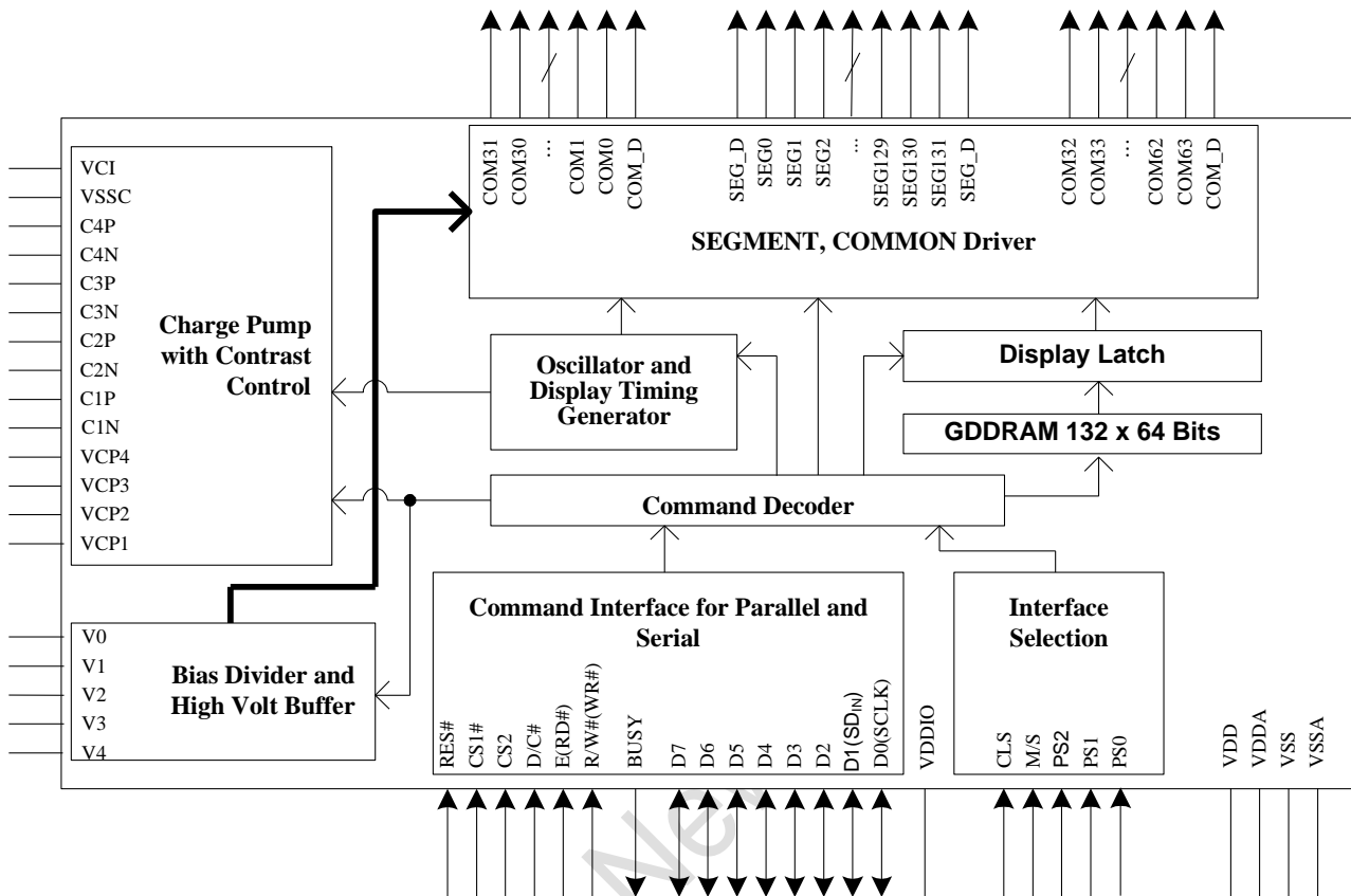
Figure 4-1 : Block Diagram
