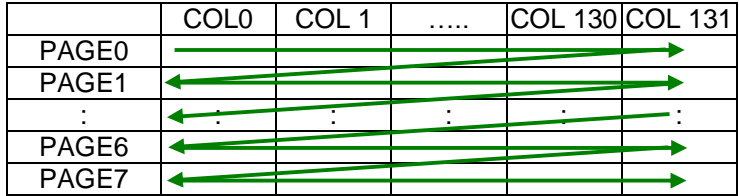
Figure 9-2 : Address Pointer Movement of Horizontal addressing mode
