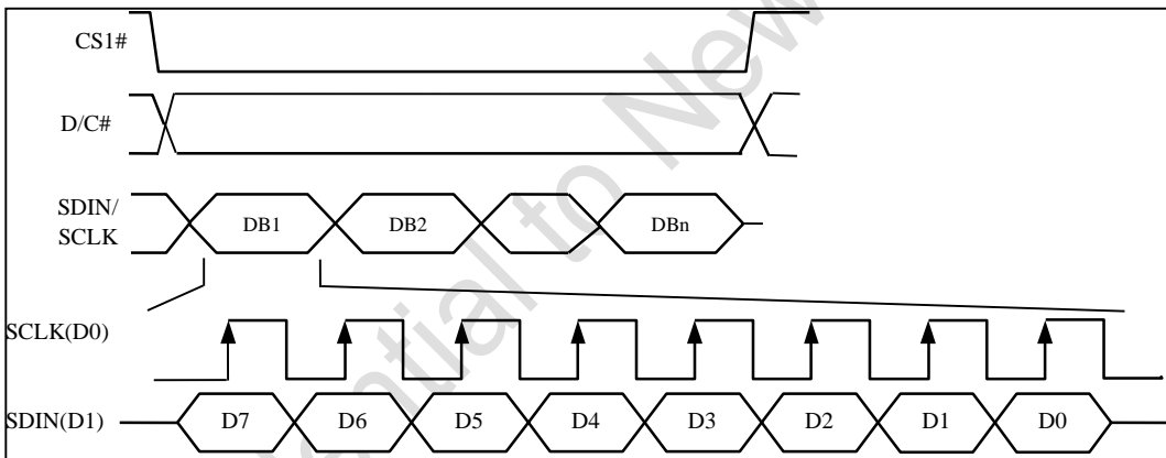
Figure 7-3 : Display data write procedure in SPI4 mode
